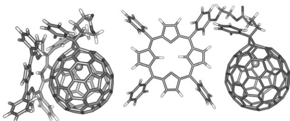
Figure 3. Two optimized conformers of M_3 Por at the M06-2X/3-21G-LanL2DZ level. The folded conformer (left) is 14.5 kcal mol −1 more stable than stretched conformer (right) at this level.
